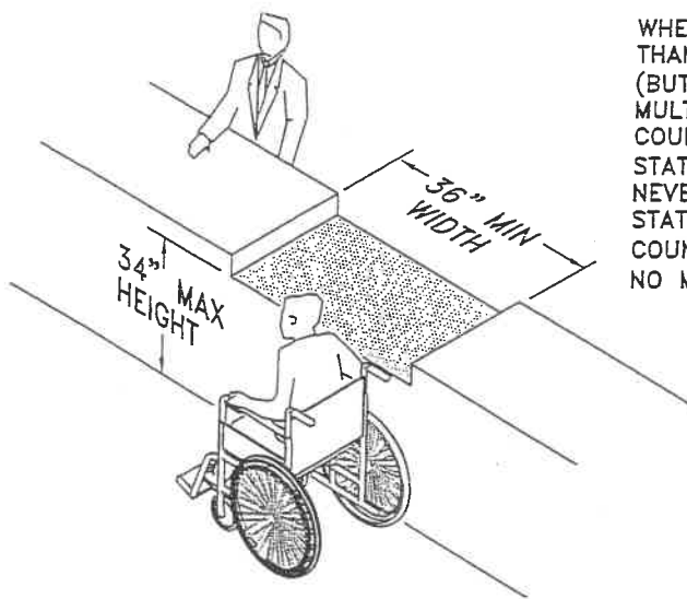
Fig. 121 MULTIPLE TRANSACTION STATIONS FIXED OR BUILT-IN SEATING, TABLES & COUNTERS
