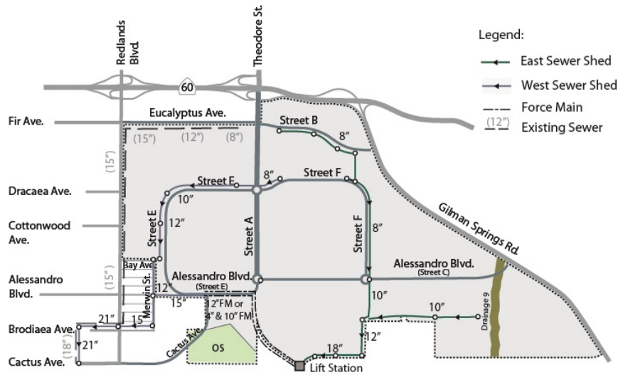
Exhibit 3-20 Wastewater Service Plan
