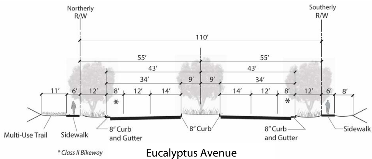
Exhibit 3-6 Street "B" (Eucalyptus Avenue Extension) (pg.3-5)
