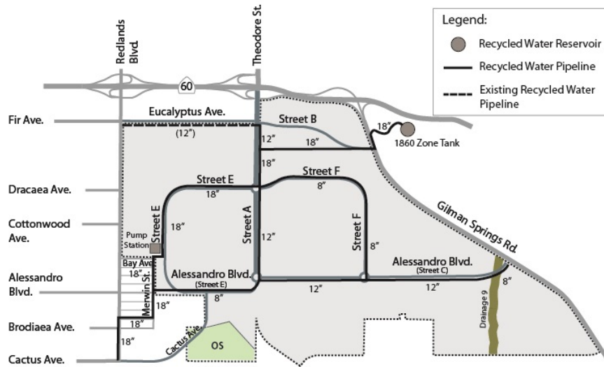
Exhibit 3-21 Recycled Water Plan
