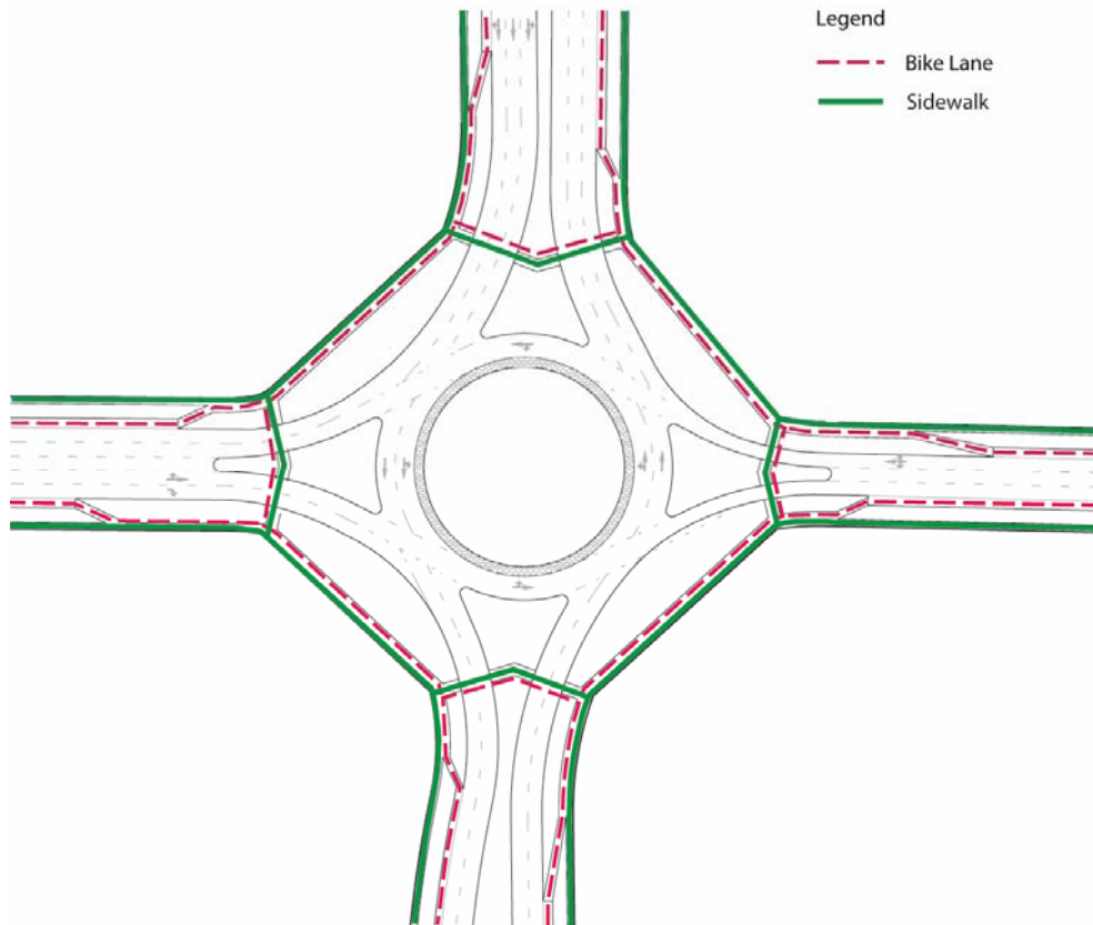
Exhibit 3-12 Roundabout Diagram
